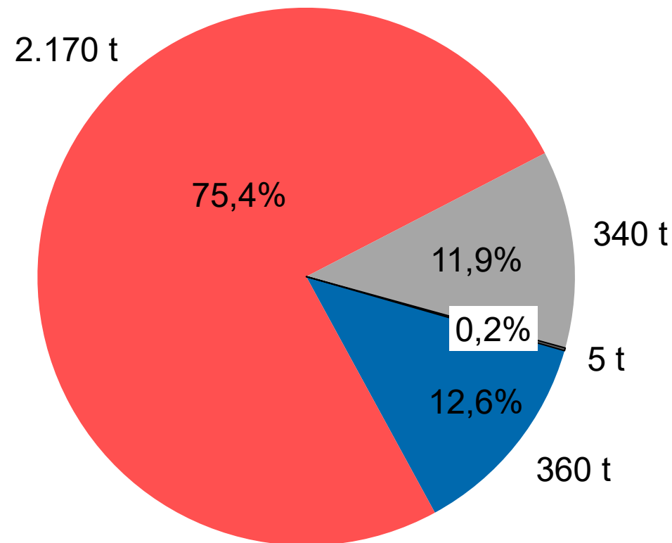
CO 2 -Bilanz 2023
